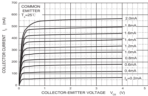
Static Characteristic
